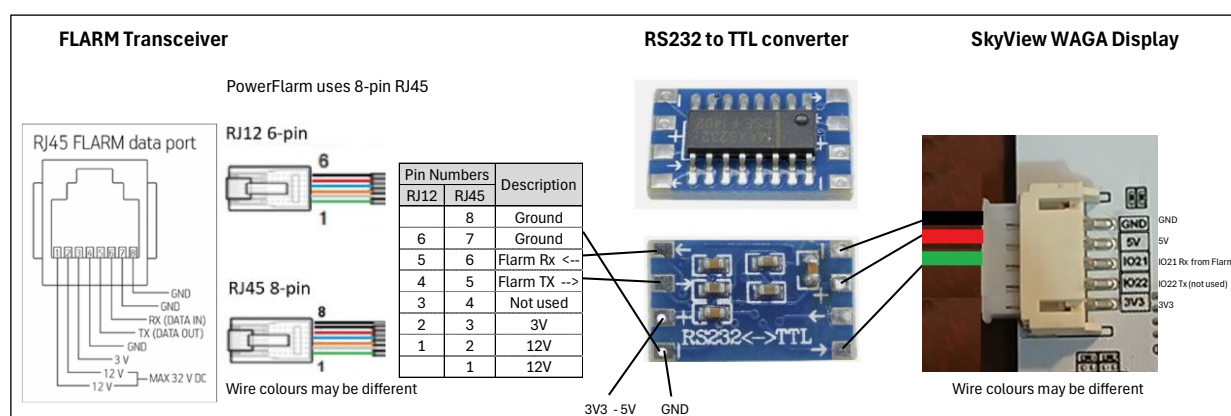
Diagram RJ45 pinout, example RS232 -> TTL board and SkyView 5-pin side connector
