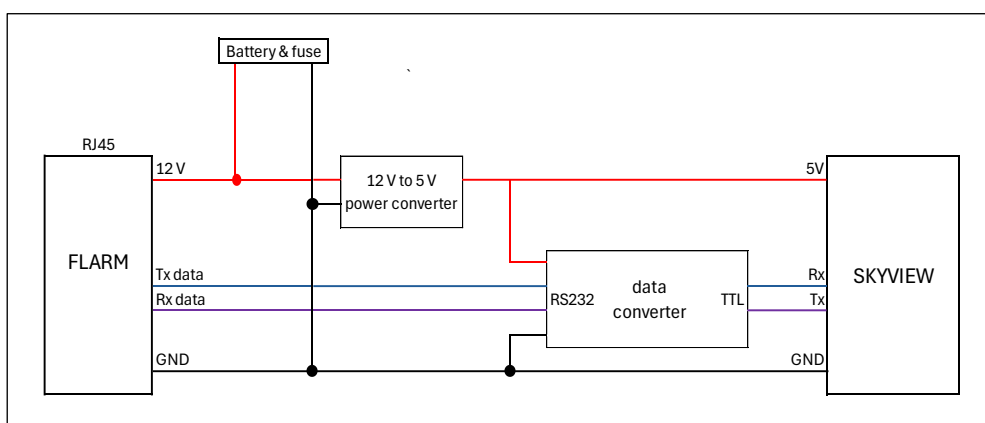
Schematic diagram of connection for a non-WAGA Flarm
